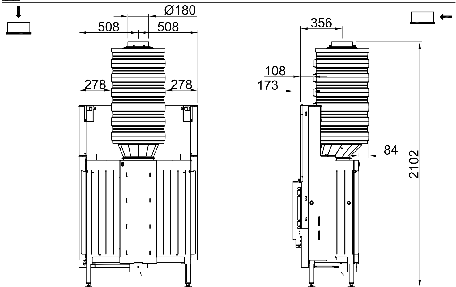
~1:20 Top outlet, eccentric adapter
